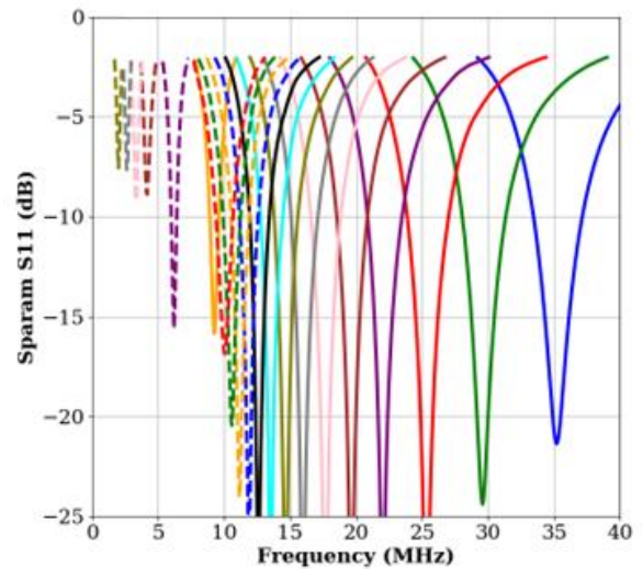
Return Loss for Various Tuned Operating Frequencies
