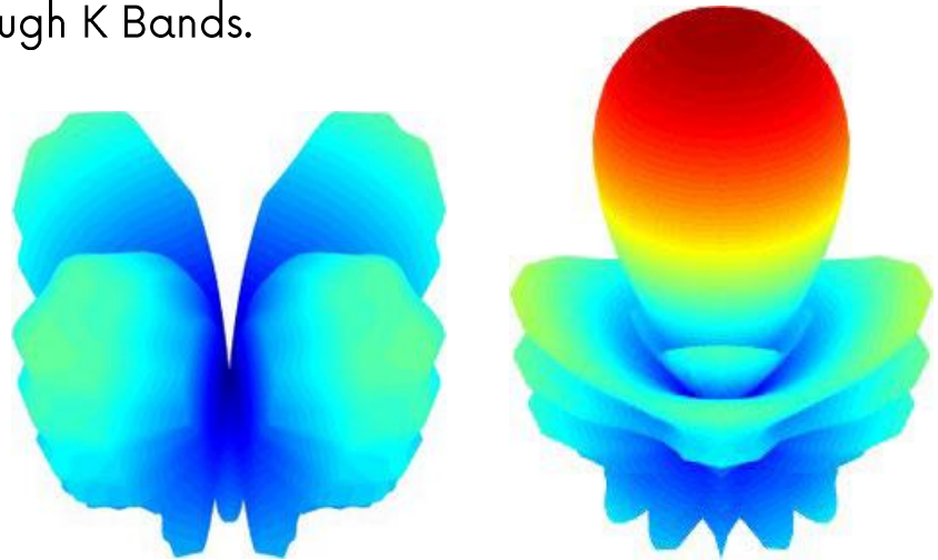
Cx-Pol Gain
